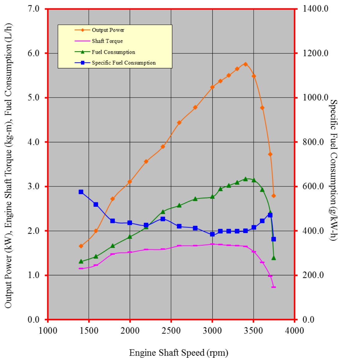
Figure 2. Performance characteristic curves of the HONDA GX270 gasoline engine (with an oil-bath type air cleaner)
