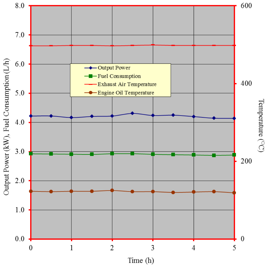
Figure 3. Performance characteristic curves during the continuous running test of the HONDA GX270 gasoline engine (with an oil-bath type air cleaner)
